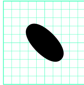
plain filled curvetrace
