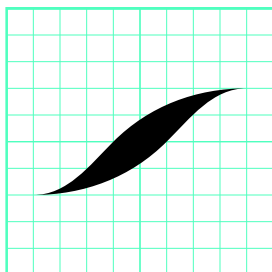
double filled curvetrace
