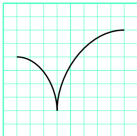
curvetrace with a cusp
