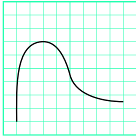
plain stroked curvetrace
