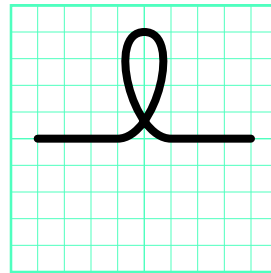
curvetrace inside a path
