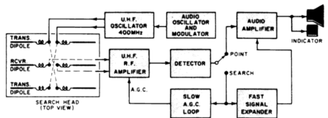
Fig. 6. U.H.F. induction-balance locator operates on metals or non-metals. Search mode eliminates spurious terrain response.
