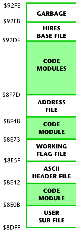
Fig. 3-9. Separating HRCG stashes from the code modules.
