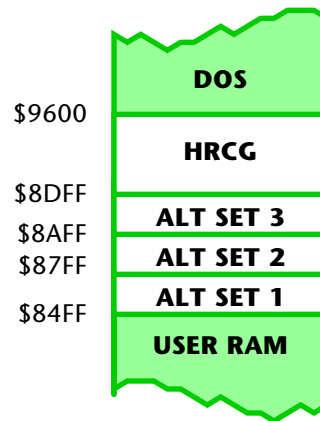
Fig. 3-7. Location of 48K Apple HRCG program and alternate character sets.
