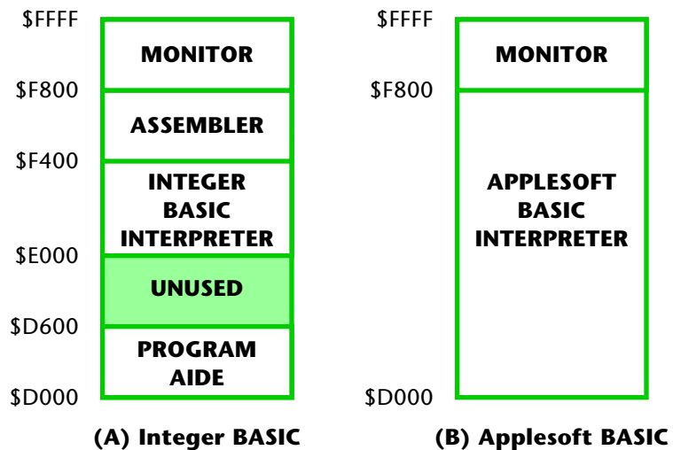
Fig. 3-6. The high ROM maps. A plug-in ROM or RAM card can deactivate these and substitute its own code.
