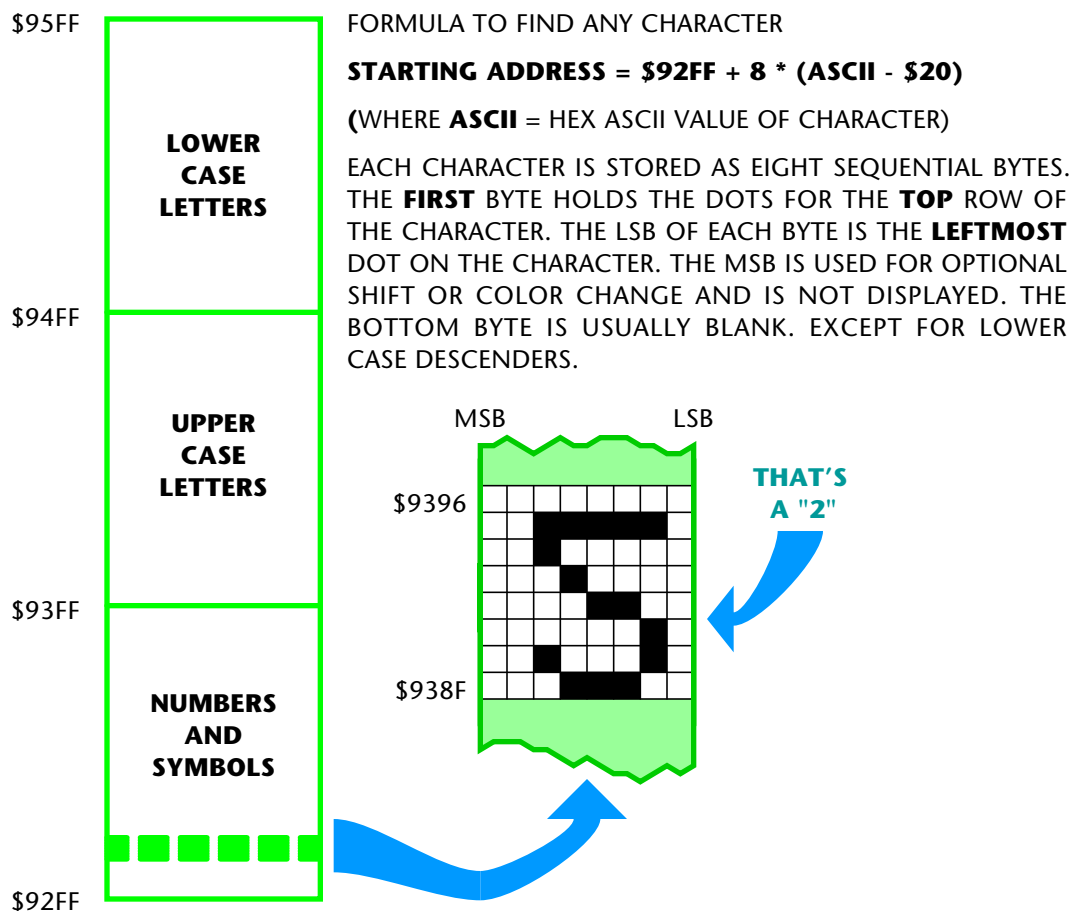
Fig. 3-10. How the HRCG character set is stored in the bulk file.
