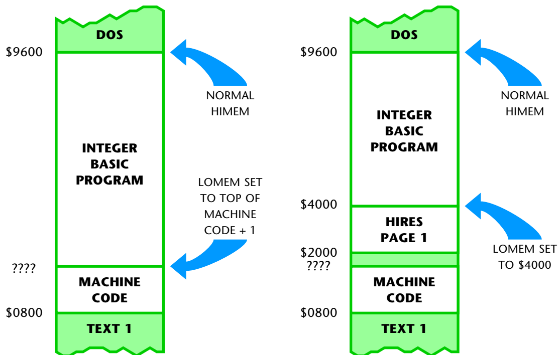
(A) Integer Basic, no HIRES
